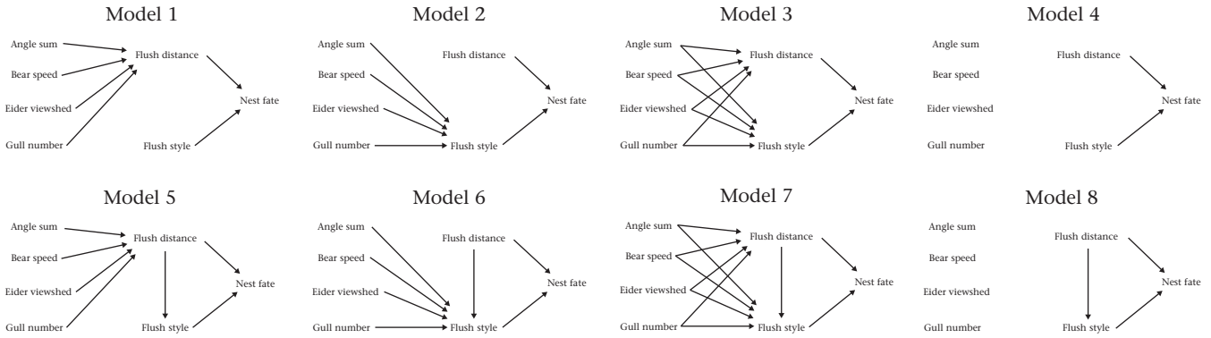
Figure 3. Candidate path diagrams relating predator and environmental cues to flushing behaviour and nest fate of common eiders. Arrows represent conceptual unidirectional relationships between variables.
